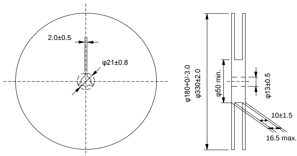
Fig.3 Taping Diagram
