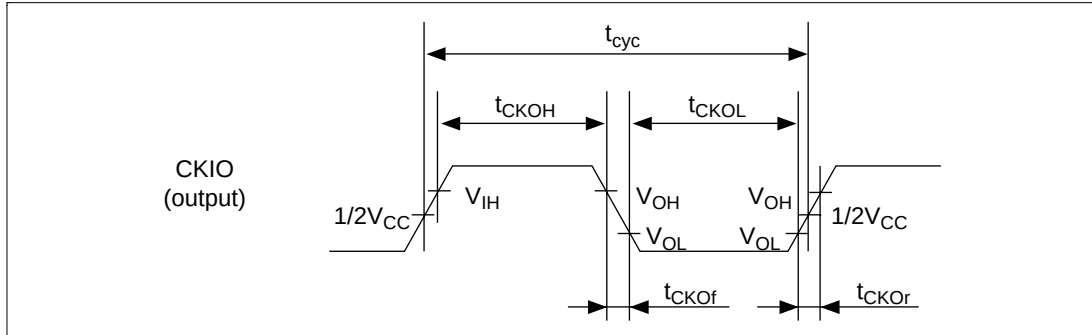
Figure 16.3 CKIO Clock Output Timing
