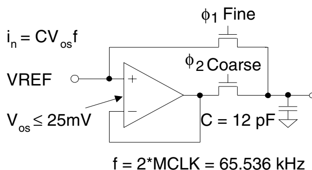
Figure 8. Input model for VREF+ and VREF- pins.
