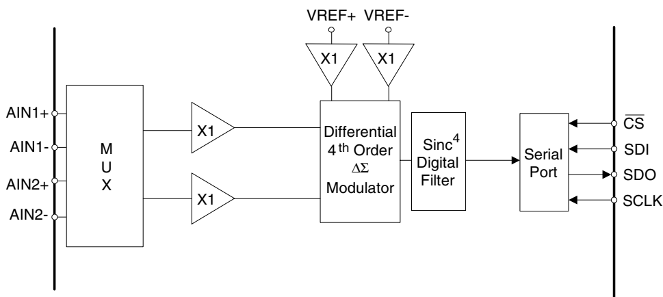
Figure 4. Multiplexer Configuration.
