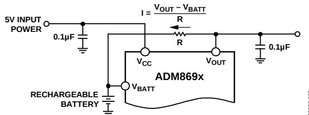
Figure 25. Rechargeable Battery
