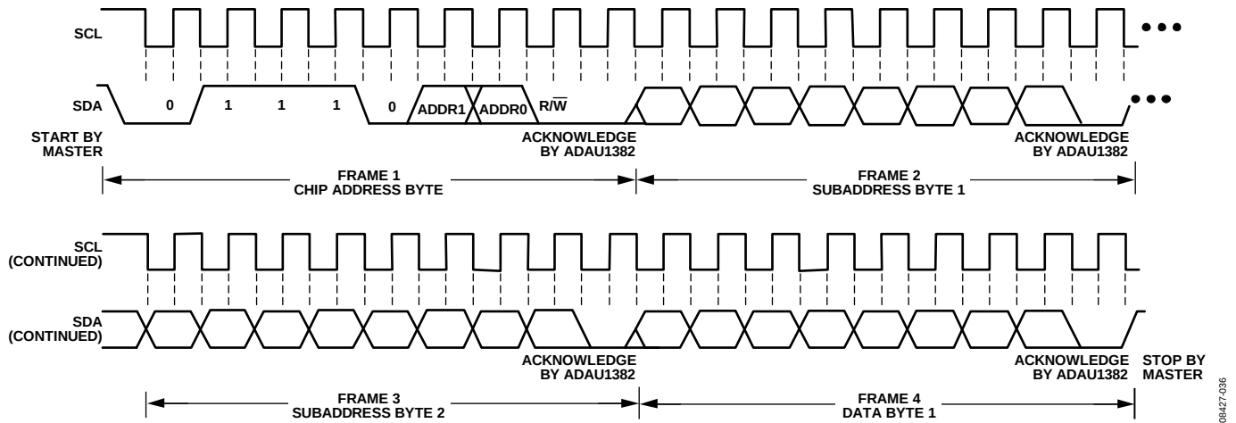
Figure 37. I²C Write to ADAU1382 Clcking
