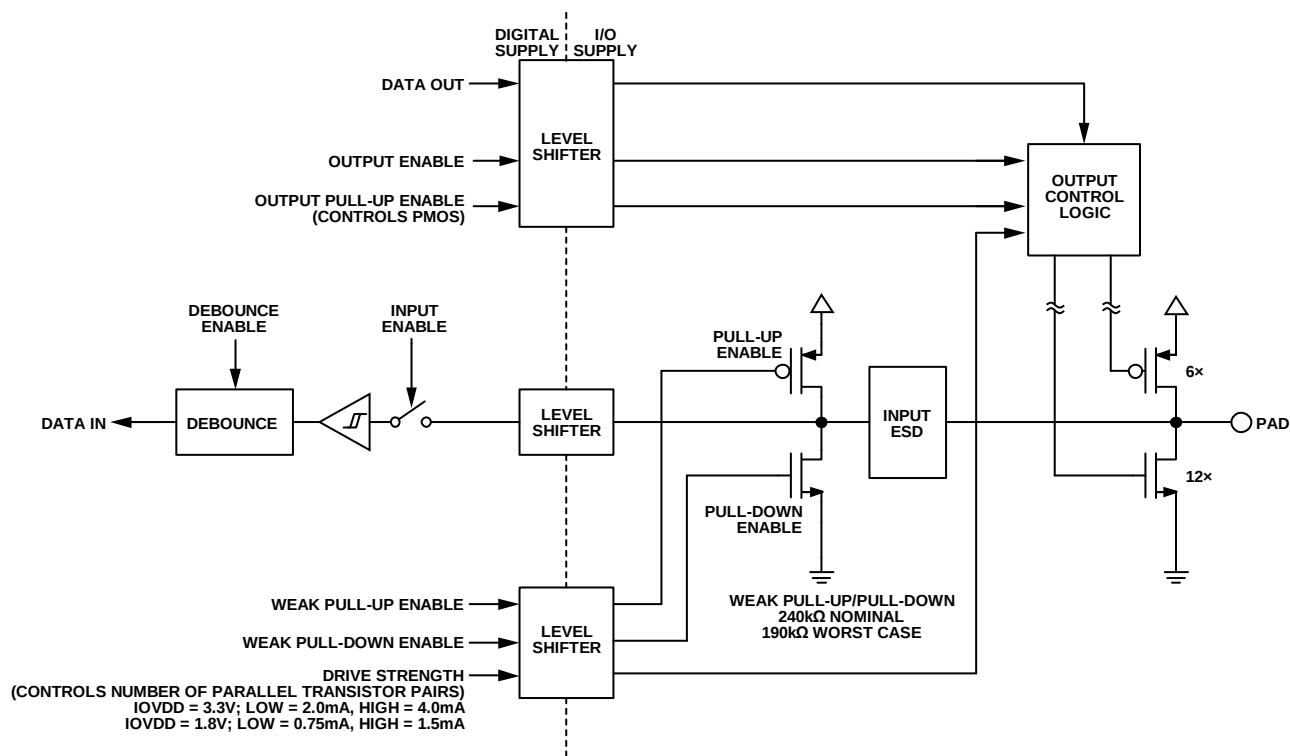
Figure 70. Pad Configuration, Internal Design
