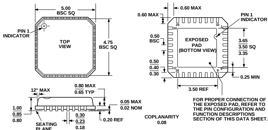
COMPLIANT TO JEDEC STANDARDS MO-220-VHHD-2 Figure 72. 32-Lead Lead Frame Chip Scale Package [LFCSP_VQ] 5 mm × 5 mm Body, Very Thin Quad (CP-32-4) Dimensions shown in millimeters
