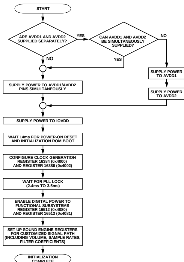
Figure 26. Initialization Sequence
