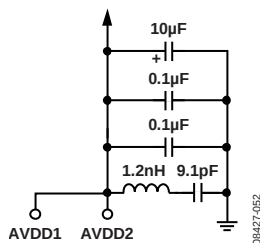
Figure 53. GSM Filter on the Analog Supply Pins
