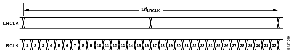
Figure 60. Example: 32 BCLK Cycles per Frame
