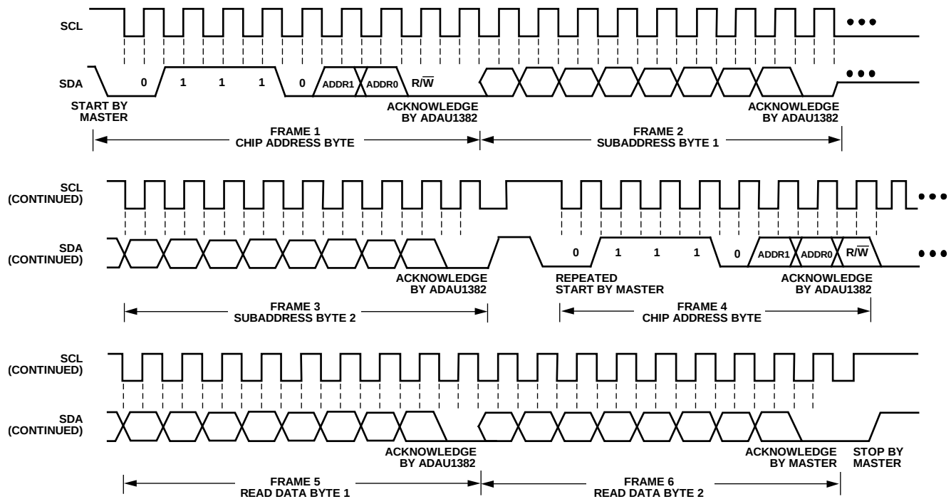
Figure 38. I²C Read from ADAU1382 Clcking
