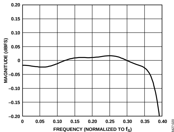
Figure 19. DAC Interpolation Filter Pass-Band Ripple, Double-Rate Mode, Normalized to f_s
