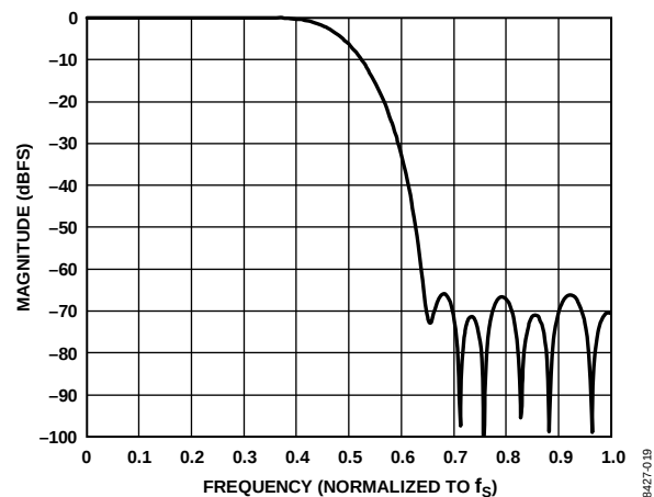
Figure 18. DAC Interpolation Filter, Double-Rate Mode, Normalized to f_s
