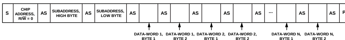
Figure 40. Burst Mode I 2 C Write Sequence
