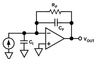
Figure 1. Transimpedance Configuration
