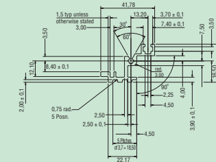
Handle Extrusion
