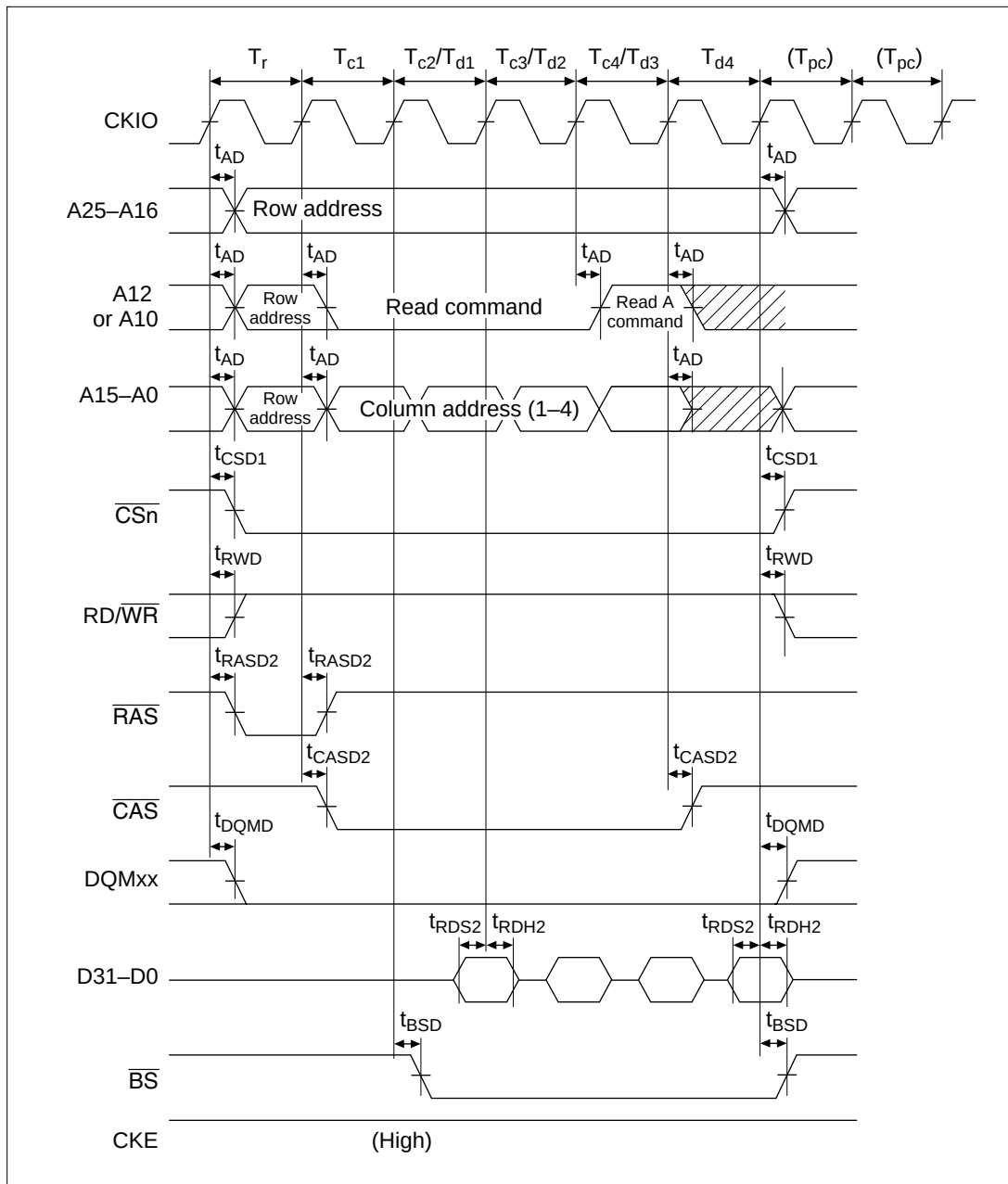
Figure 16.36 Synchronous DRAM Read Bus Cycle (Burst Read (Single Read \times 4), RCD = 0, CAS Latency = 1, TPC = 1)
