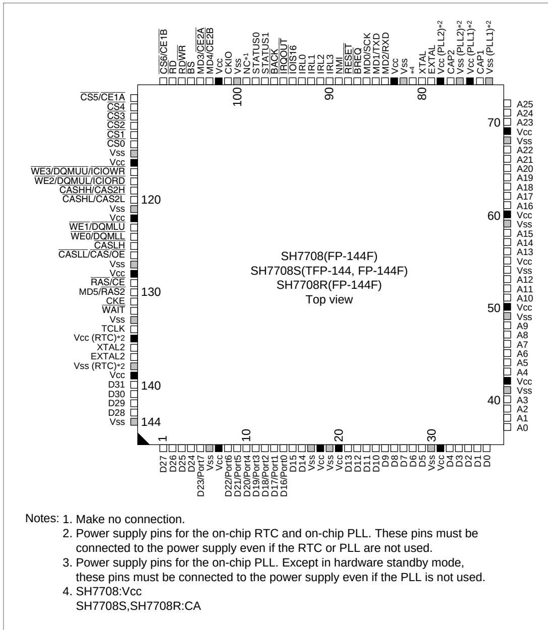
Figure 1.2 Pin Arrangement
