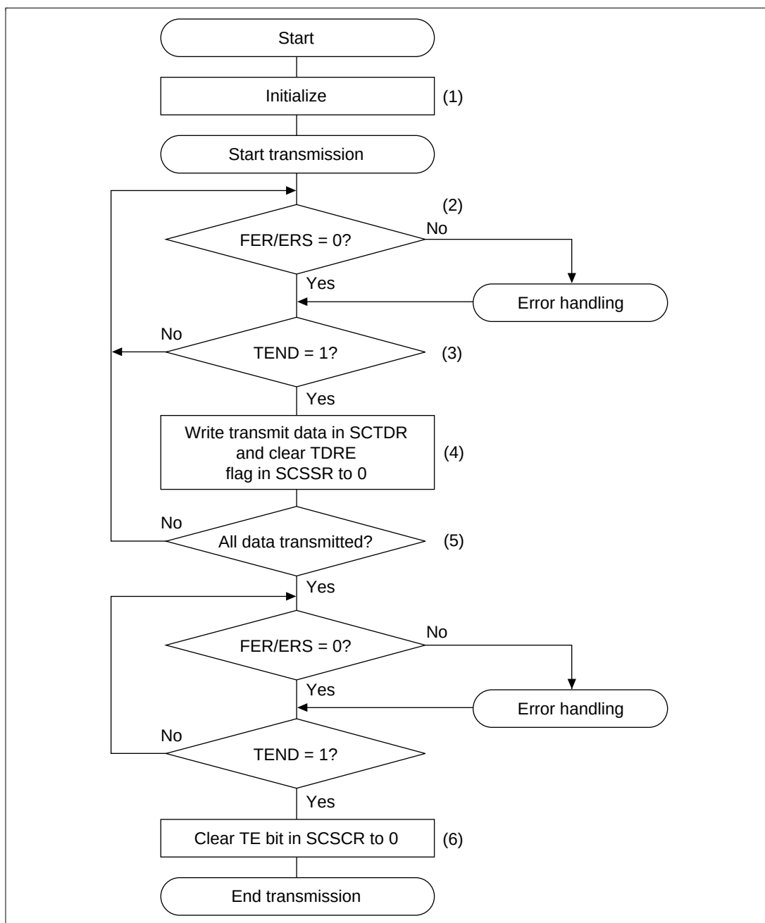
Figure 14.6 Transmission Flowchart
