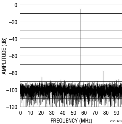
LTC2220-1: 8192 Point FFT, f_{IN} = 500\text{MHz} , -6dB, 1V Range, LVDS Mode
