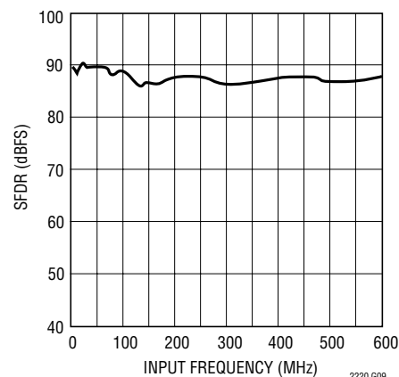
LTC2220-1: SFDR (HD4+) vs Input Frequency, -1dB, 1V Range, LVDS Mode
