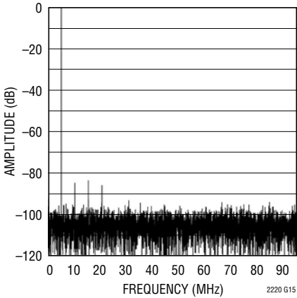
LTC2220-1: 8192 Point FFT, f_{IN} = 5\text{MHz} , -1dB, 2V Range, LVDS Mode
