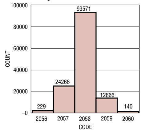
LTC2220-1: Shorted Input Noise Histogram
