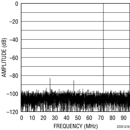
LTC2220-1: 8192 Point FFT, f_{IN} = 70\text{MHz} , -1dB, 2V Range, LVDS Mode
