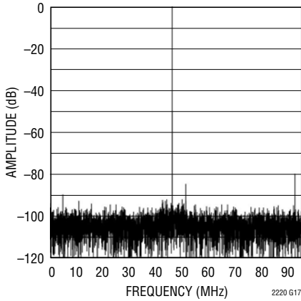
LTC2220-1: 8192 Point FFT, f_{IN} = 140\text{MHz} , -1dB, 2V Range, LVDS Mode
