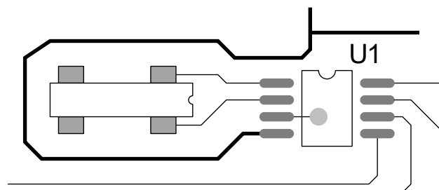
FIGURE 15. SUGGESTED LAYOUT FOR ISL12057 AND CRYSTAL
