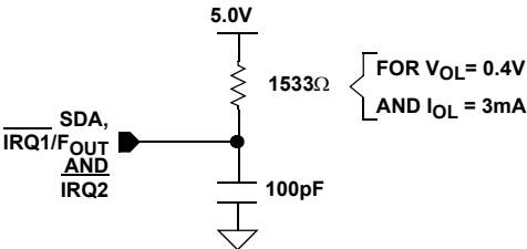
FIGURE 4. STANDARD OUTPUT LOAD FOR TESTING THE DEVICE WITH V_{DD} = 5.0V
