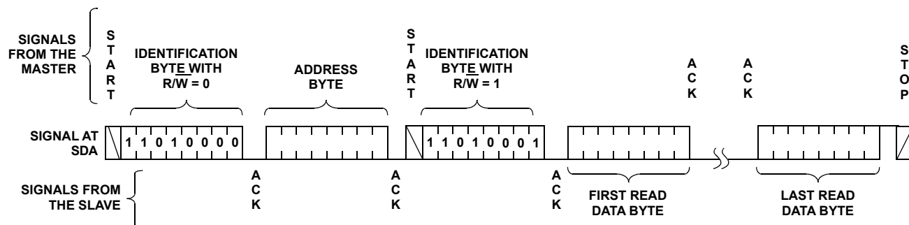
FIGURE 14. READ SEQUENCE
