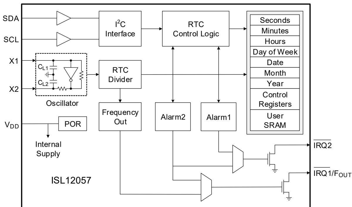
FIGURE 3. BLOCK DIAGRAM
