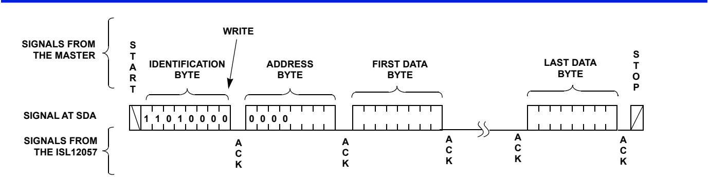
FIGURE 12. SEQUENTIAL BYTE WRITE SEQUENCE
