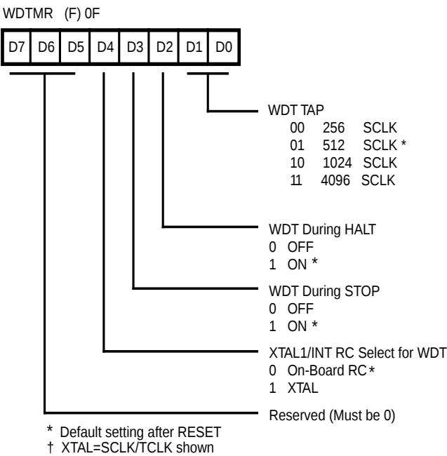
Figure 49. Watch-Dog Timer Mode Register (Write-Only)
