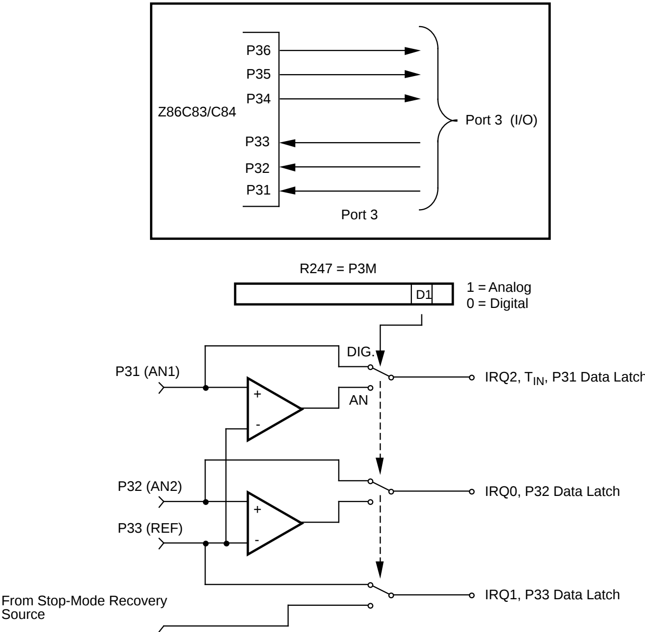
Figure 12. Port 3 Input Configuration
