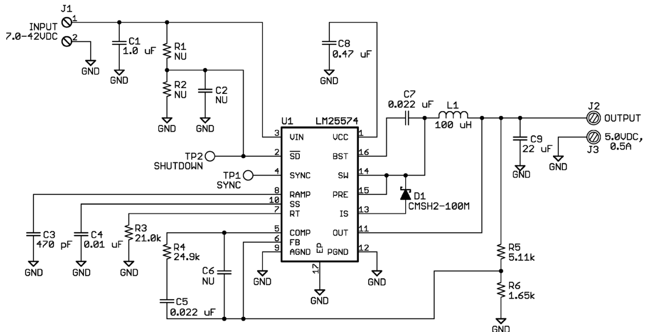
Figure 7-1. LM25574 Reference Schematic
