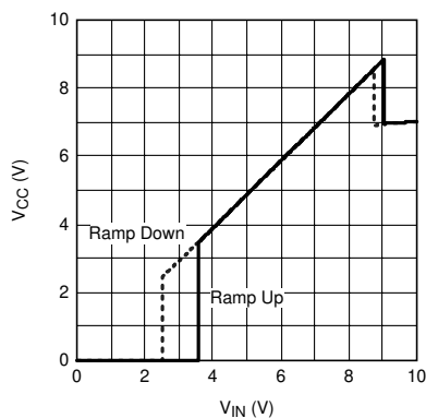
Figure 5-5. V_{CC} vs V_{IN}
