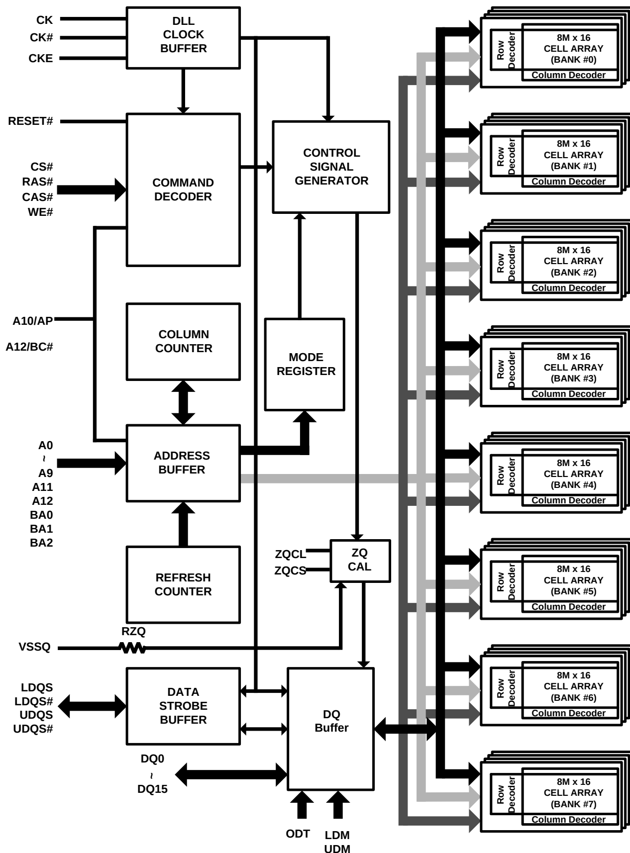
Figure 2. Block Diagram
