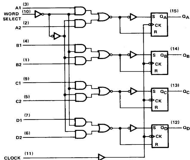
logic diagram
