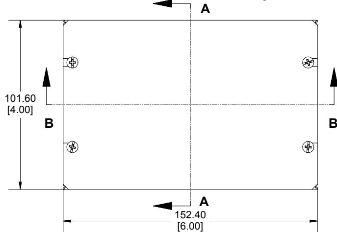
Bottom View of Assembly
