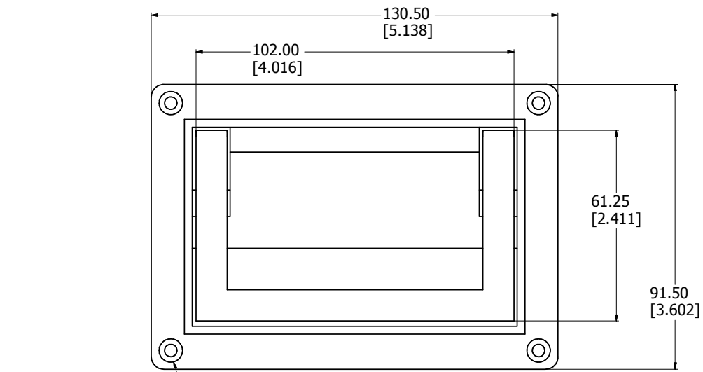
FRONT VIEW
