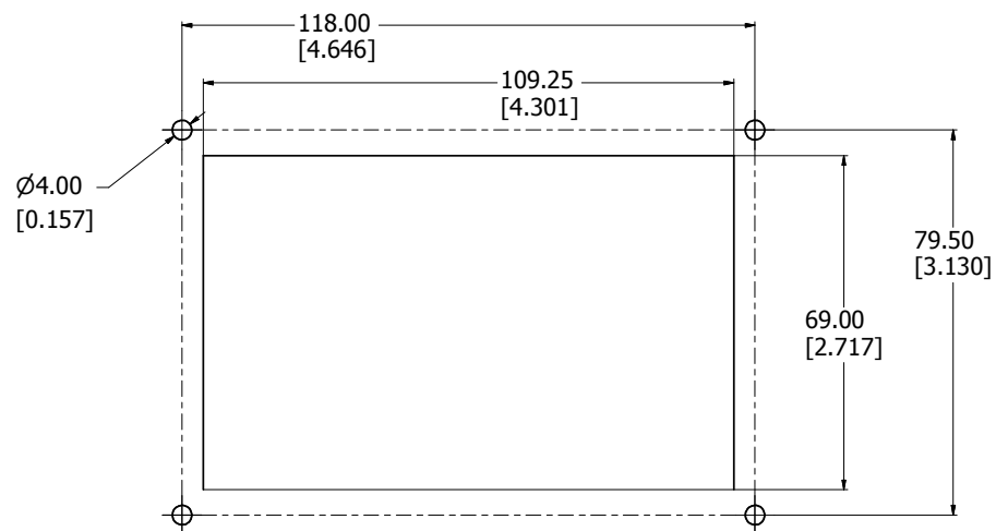
MOUNTING OPENING
