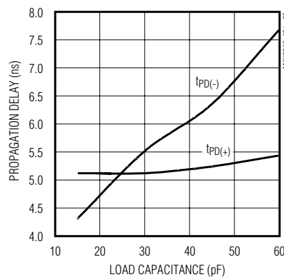
PROPAGATION DELAY vs. LOAD CAPACITANCE
