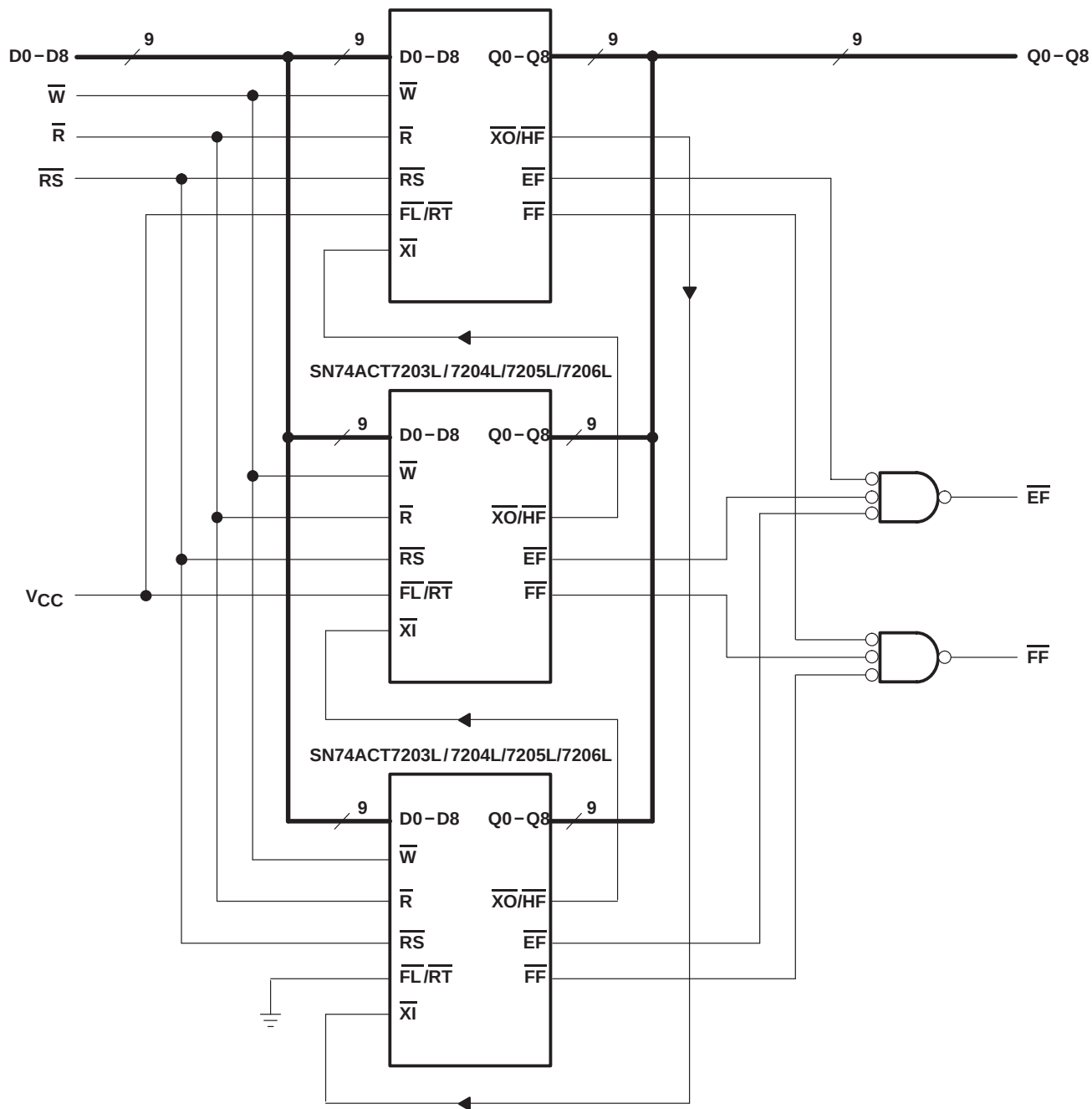
Figure 15. Word-Depth Expansion: 6144/12288/24576/49152 Words \times 9 Bits
