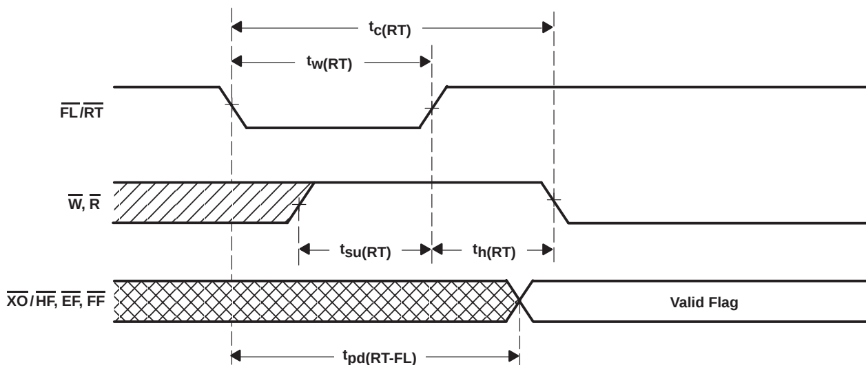
Figure 4. Retransmit Waveforms
