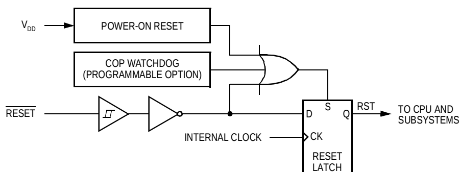
Figure 5-1. Reset Sources
