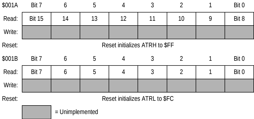
Figure 9-14. Alternate Timer Registers (ATRH and ATRL)
