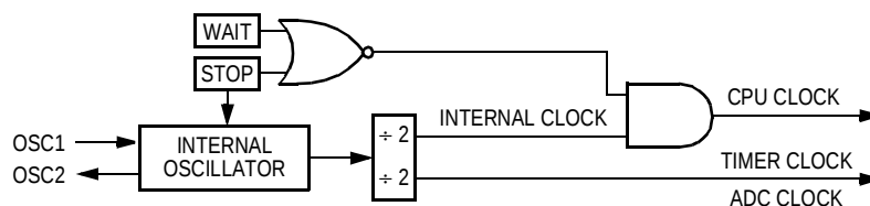
Figure 6-4. STOP/WAIT Clock Logic
