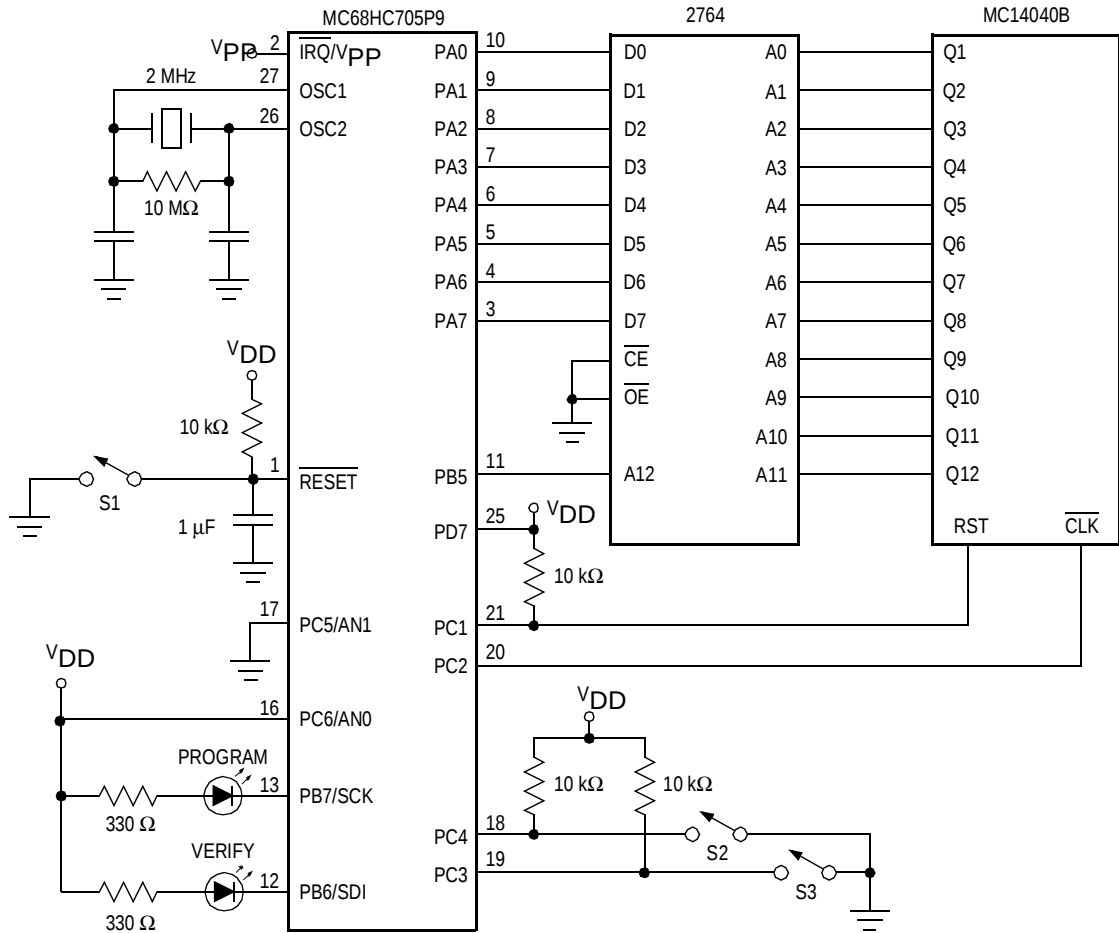
Figure 3-4. Bootloader Circuit
