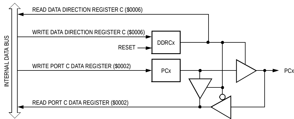
Figure 7-10. Port C I/O Logic
