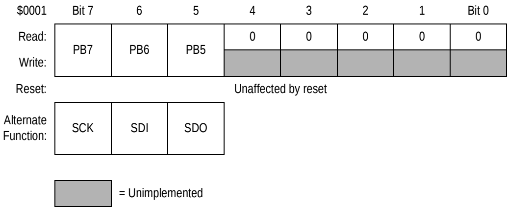
Figure 7-5. Port B Data Register (PORTB)
