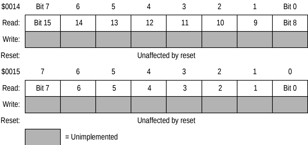
Figure 9-16. Input Capture Registers (ICRH and ICRL)
