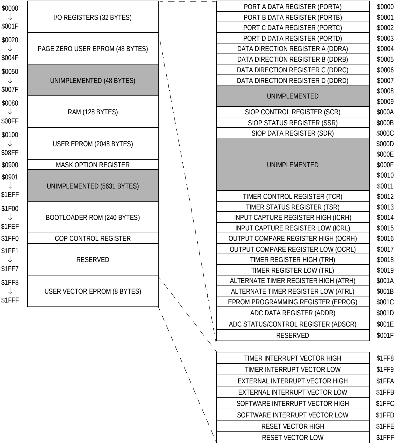
Figure 3-1. Memory Map
