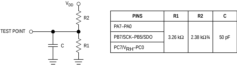
Figure 12-5. Test Load
