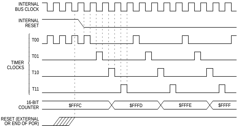
Figure 9-6. Timer Reset Timing
