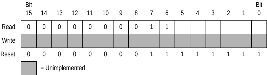
Figure 4-4. Stack Pointer (SP)
