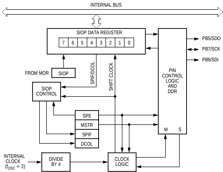
Figure 10-1. SIOP Block Diagram
