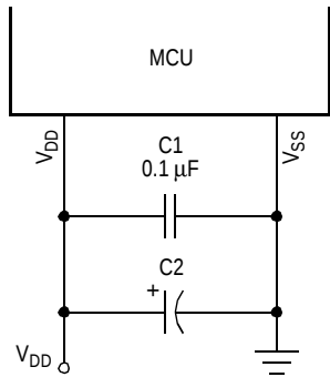
Figure 2-2. Bypassing Recommendation
