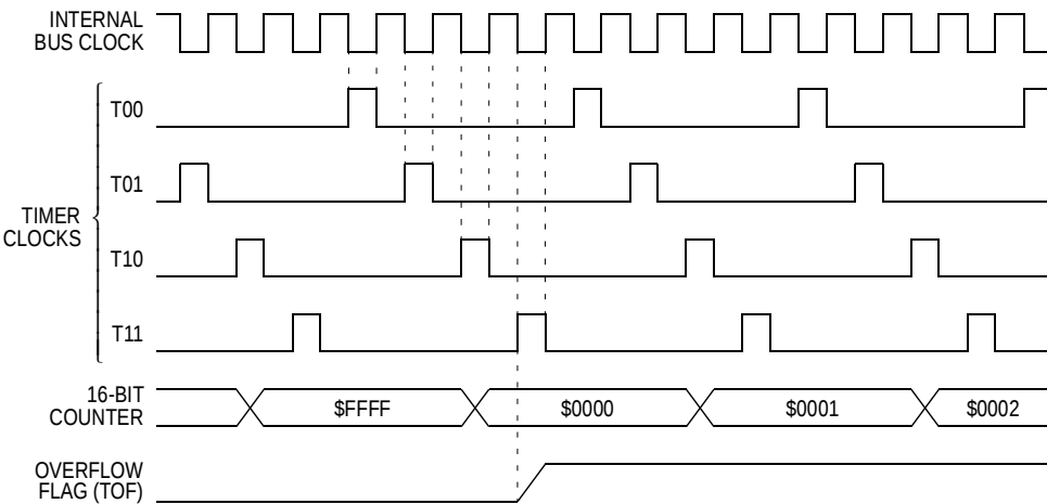
Figure 9-9. Timer Overflow Timing
