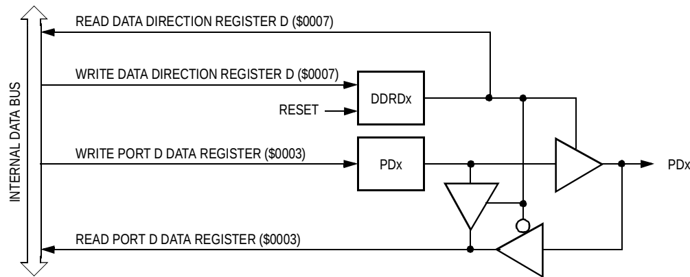
Figure 7-13. Port D I/O Logic
