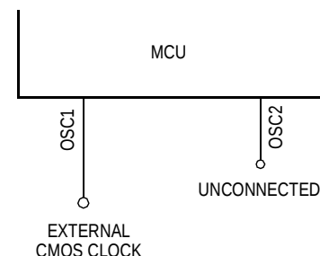
Figure 2-5. External Clock Connections
