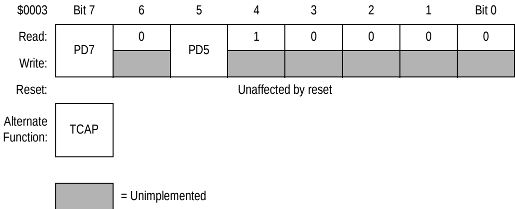
Figure 7-11. Port D Data Register (PORTD)
