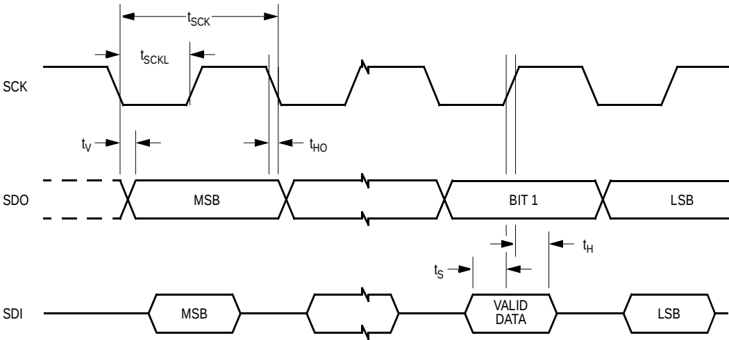
Figure 10-5. SIOP Timing
