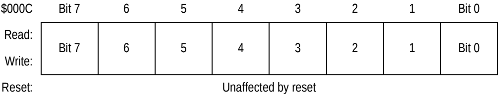
Figure 10-8. SIOP Data Register (SDR)
