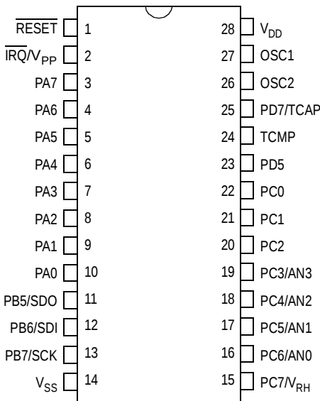
Figure 2-1. Pin Assignments
