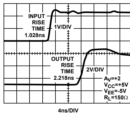
FIGURE 8. OUTPUT RISE TIME
