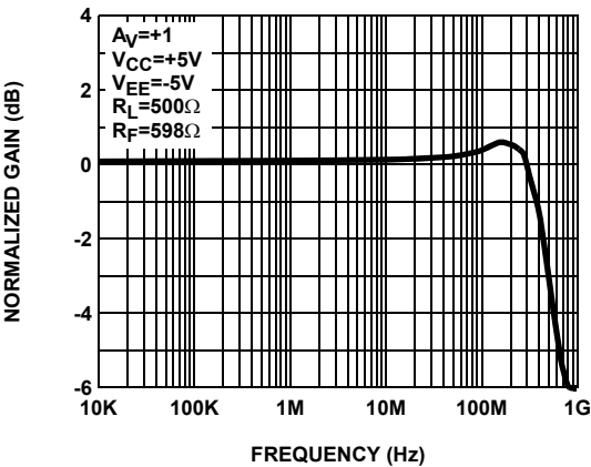
FIGURE 1. FREQUENCY RESPONSE FOR A_V=+1
