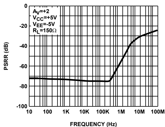
FIGURE 12. PSRR (VCC)
