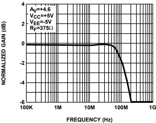
FIGURE 2. FREQUENCY RESPONSE FOR A_V=+4.6
