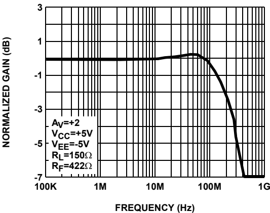
FIGURE 4. FREQUENCY RESPONSE FOR A_V=+2
