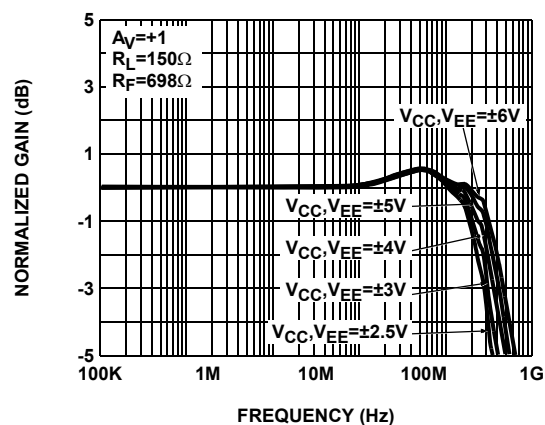
FIGURE 6. FREQUENCY RESPONSE FOR VARIOUS V_{CC} , V_{EE}
