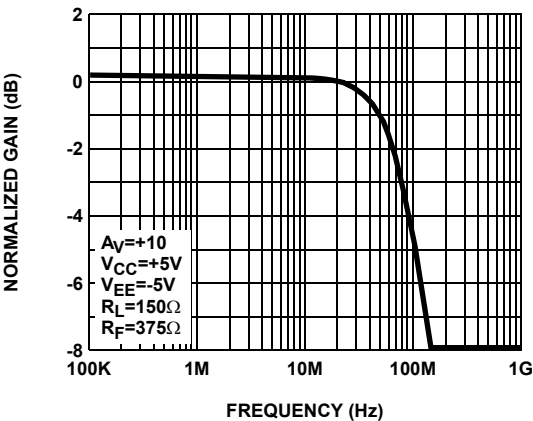
FIGURE 3. FREQUENCY RESPONSE FOR A_V=+10
