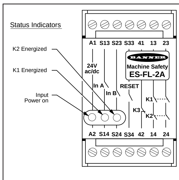
Figure 1. ES-FL-2A Status Indicators
