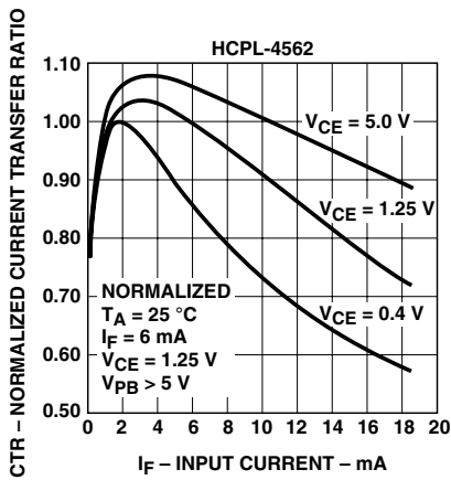
Figure 9. Current transfer ratio vs. input current
