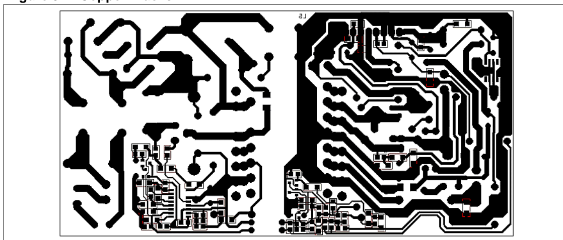
Figure 31. Copper Tracks
