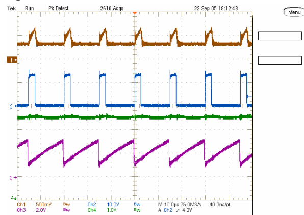
Figure 7. V_{in} = 220 \text{ Vrms} - 50\text{Hz}
