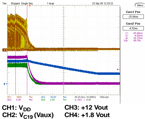
Figure 16. at 115 V AC - 60Hz
