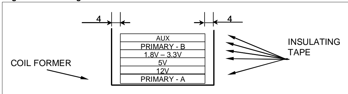
Figure 33. Winding Position
