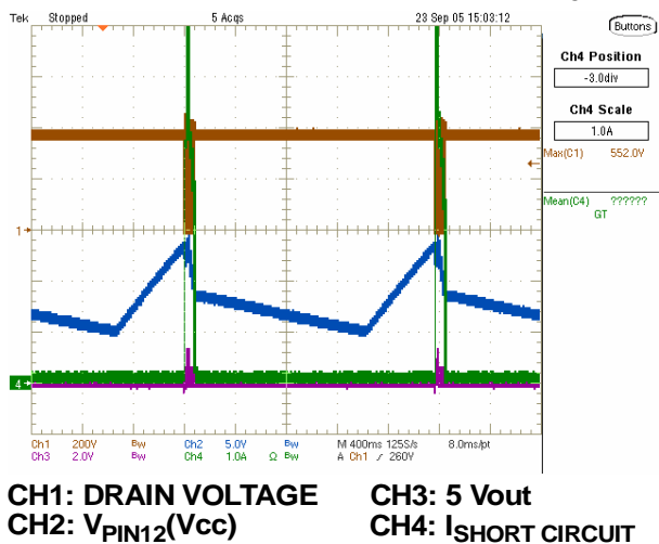
Figure 21. 5V OUTPUT SHORT at 265 V AC
