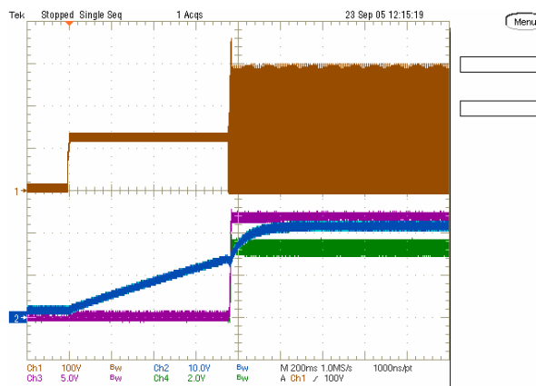
Figure 14. at 115 V AC - 60Hz
