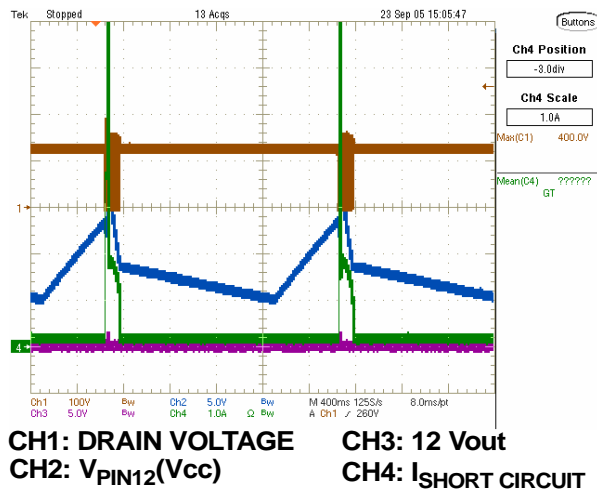
Figure 18. 12V OUTPUT SHORT at 90 V AC
