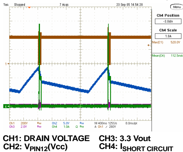
Figure 20. 3.3V OUTPUT SHORT at 265 V AC
