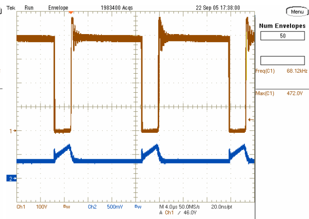
Figure 4. V_{in} = 230 \text{ Vrms} - 50\text{Hz}
