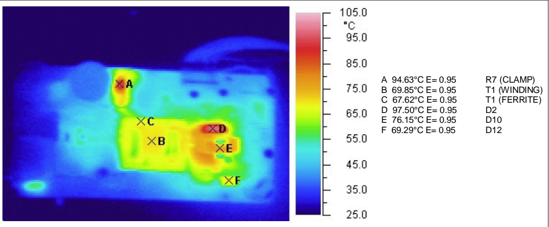
Figure 28. 230Vac-Max Load
