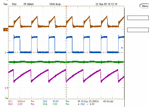
Figure 6. V_{in} = 115 \text{ Vrms} - 60\text{Hz}
