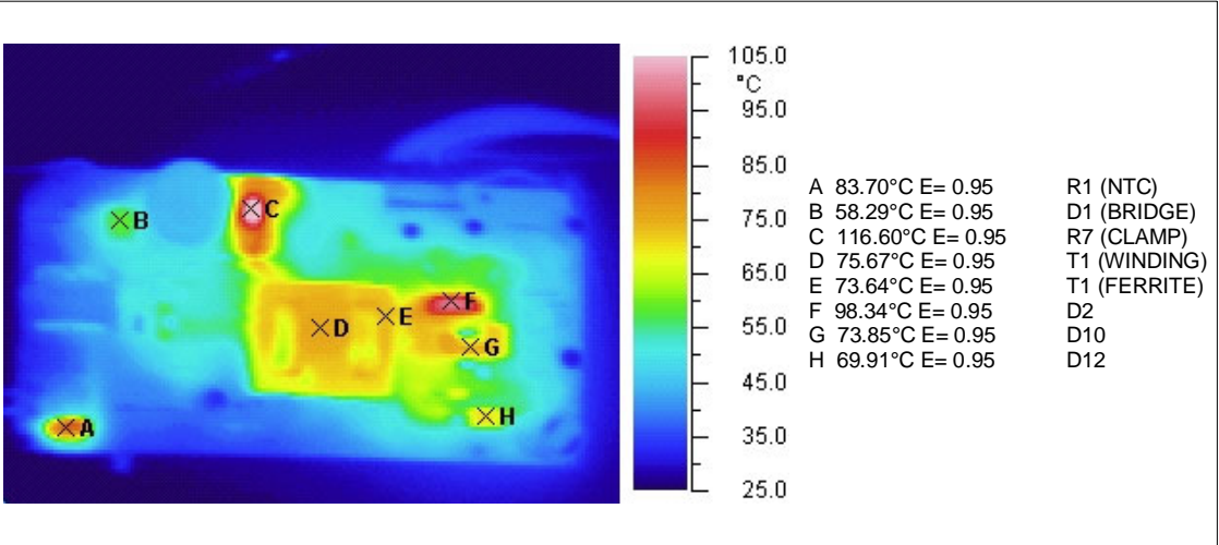
Figure 27. 115Vac-Max Load
