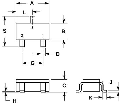
CASE 318D-04 ISSUE F SC-59
