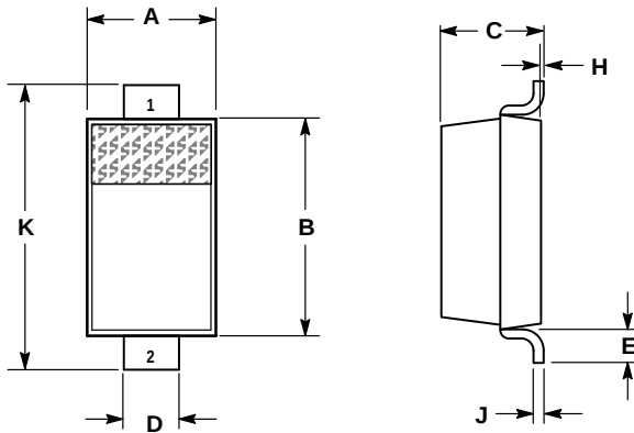
CASE 425-04 ISSUE C SOD-123
