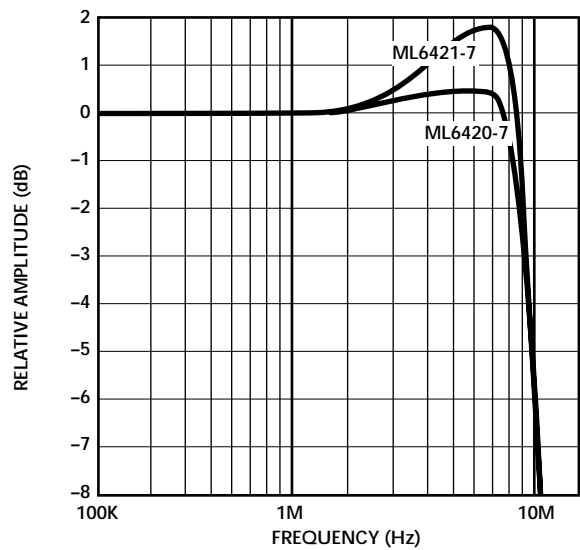
Figure 5. Pass-Band Amplitude vs Frequency ( f_C = 9.3\text{MHz} ).
