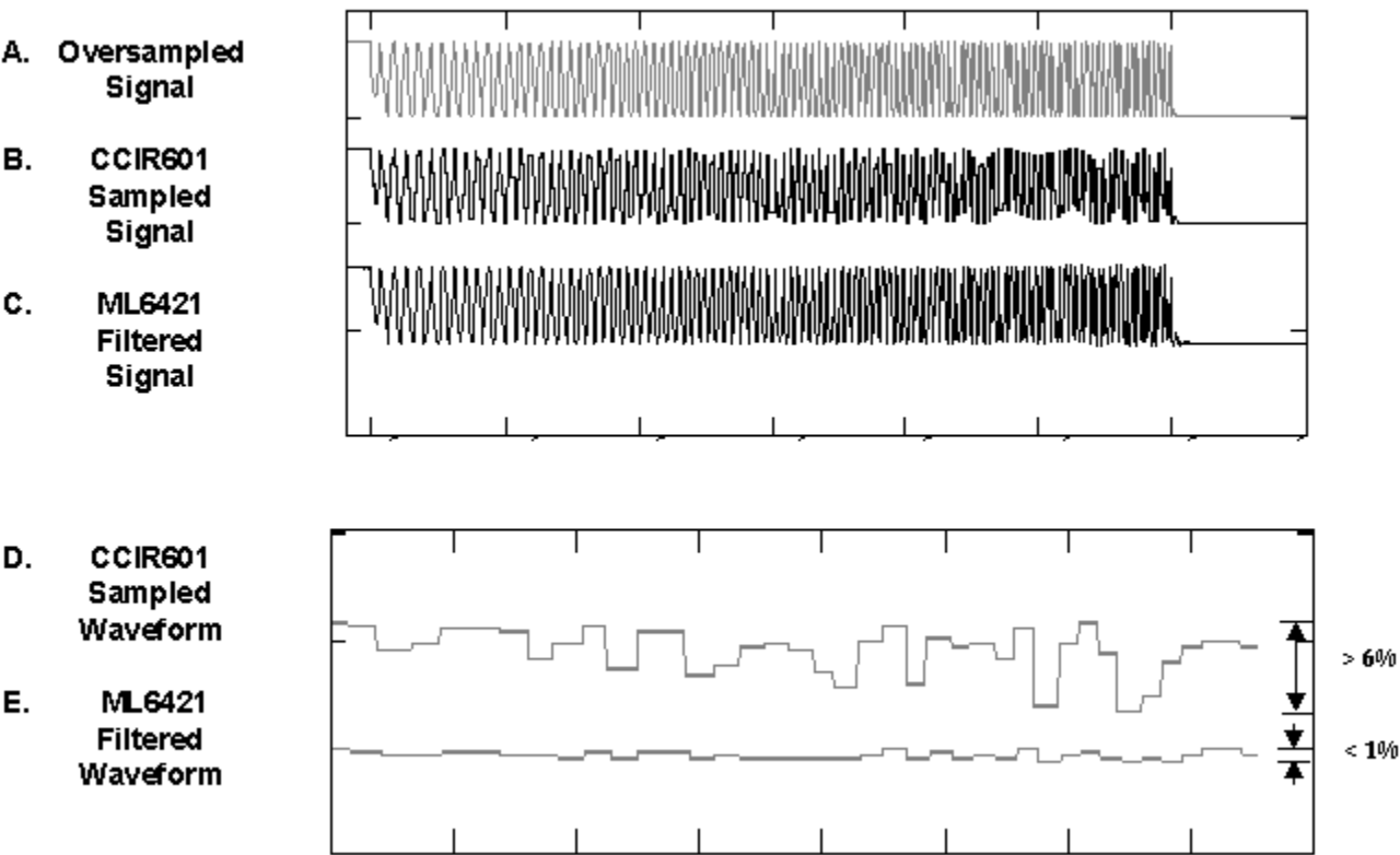
Figure 14. Amplitude Ripple of Reconstructed Swept Pulses
