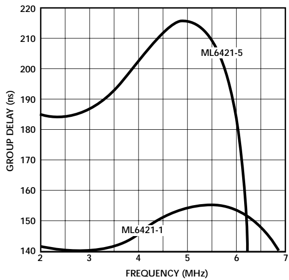
Figure 6. Group Delay vs Frequency ( f_C = 5.5\text{MHz} ).
