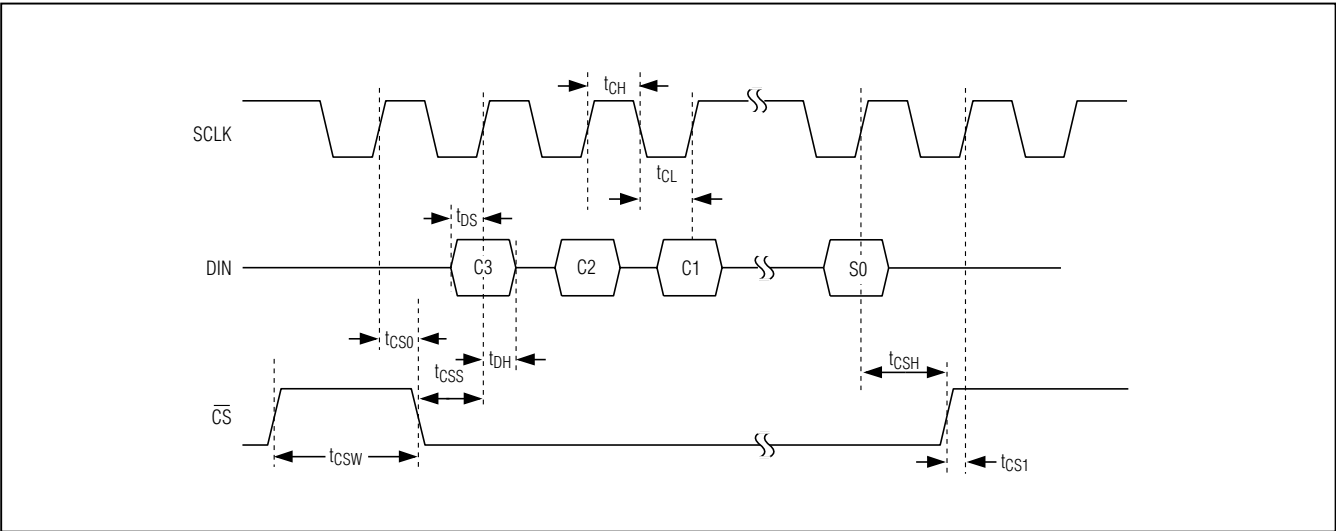
Figure 1. Timing Diagram
