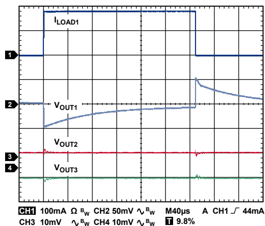
Figure 41. Load Transient Response, I_{LOAD1} = 1 \text{ mA to } 200 \text{ mA} , I_{LOAD2} = I_{LOAD3} = 1 \text{ mA} , CH1 = I_{LOAD1} , CH2 = V_{OUT1} , CH3 = V_{OUT2} , CH4 = V_{OUT3} , V_{RIPPLE} = 50 \text{ mV} , C_{OUT} = 1 \mu\text{F}
