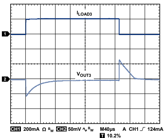
Figure 44. Load Transient Response, I_{LOAD3} = 1 \text{ mA to } 200 \text{ mA} , C_{OUT3} = 1 \mu\text{F} , CH1 = I_{LOAD3} , CH2 = V_{OUT3} , V_{RIPPLE} = 50 \text{ mV} , C_{OUT} = 1 \mu\text{F}
