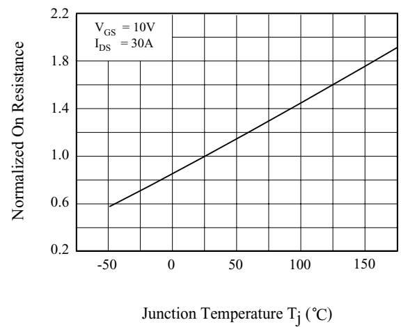
Fig 4. R_{DS(ON)} - T_j
