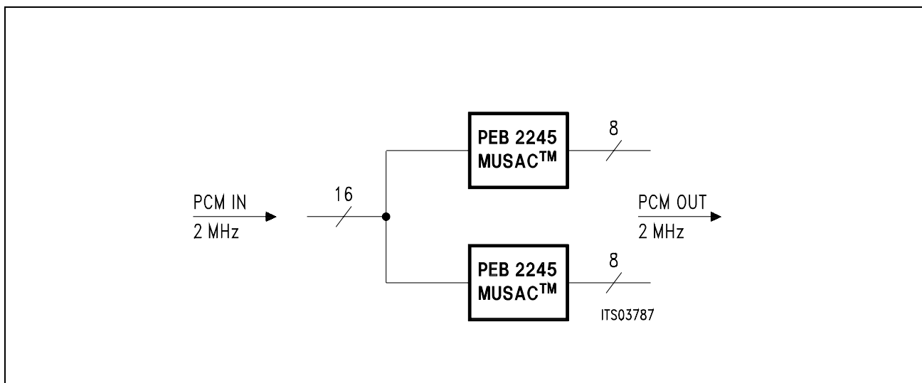
Figure 6 Memory Time Switch 16/16 for a Non-Blocking 512-Channel Switch with Conferencing Capability
