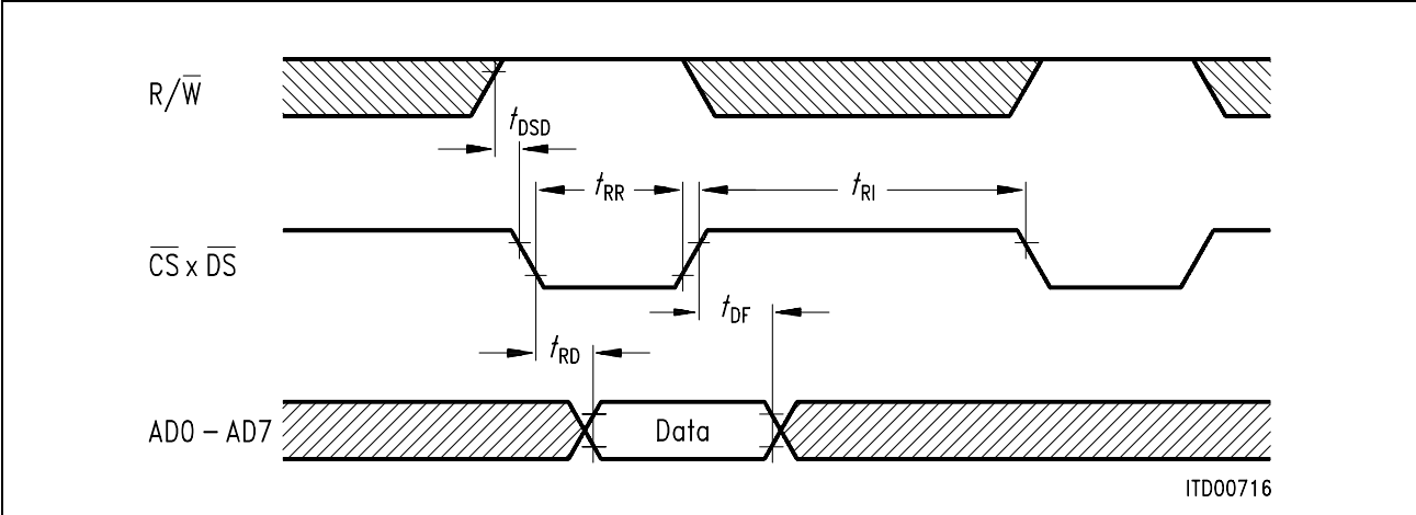
Figure 22 \mu P Write Cycle
