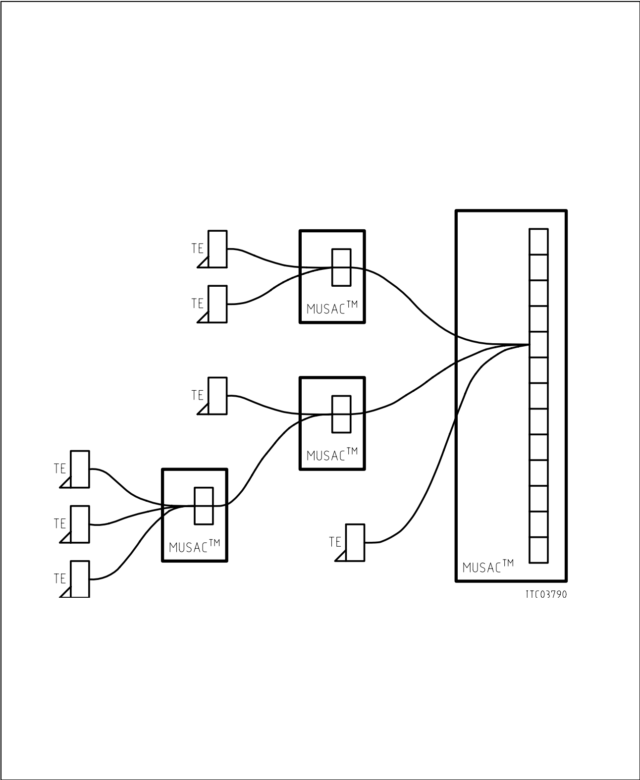
Figure 9 Multistage Arrangement
