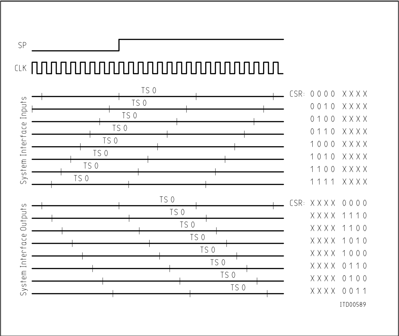
Figure 19 Clock Shifting
