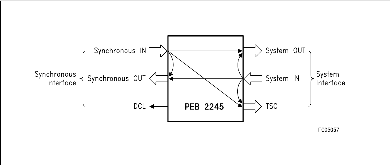
Figure 14 Connection Choices in the Primary Access Configuration
