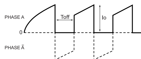
Fig.1 Constant current wave form (Motor current)
