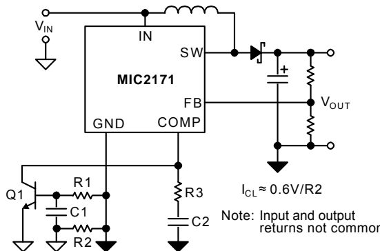
Figure 4. Current Limit
