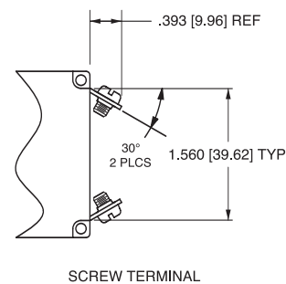
SCREW TERMINAL WITH 30° BEND
