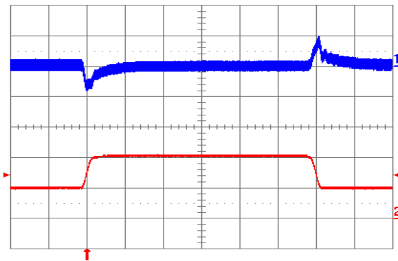
Fig. 1.5V.5: Output voltage response to load current step-change (5 A – 10 A – 5 A) at V_{in} = 48 V. Top trace: output voltage (100 mV/div.). Bottom trace: load current (5 A/div.). Current slew rate: 0.1 A/ \mu s. C_o = 1 \mu F ceramic. Time scale: 0.2 ms/div.
