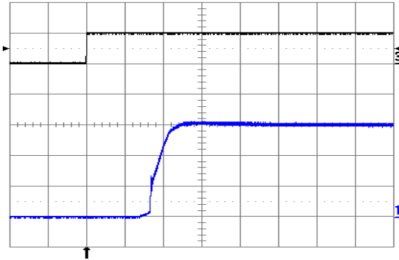
Fig. 1.5V.3: Turn-on transient at full rated load current (resistive) with no output capacitor at V_{in} = 48 V, triggered via ON/OFF pin. Top trace: ON/OFF signal (5 V/div.). Bottom trace: output voltage (0.5 V/div.). Time scale: 1 ms/div.
