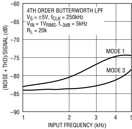
LTC1067-50 Noise + THD vs Input Frequency
