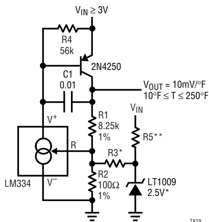
Ground Referred Fahrenheit Thermometer
