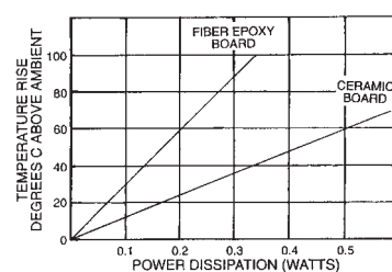
POWER DISSIPATION
