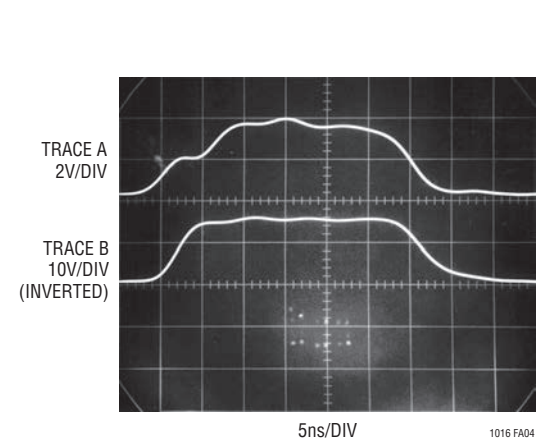
Figure A4. Figure A3's Waveforms
