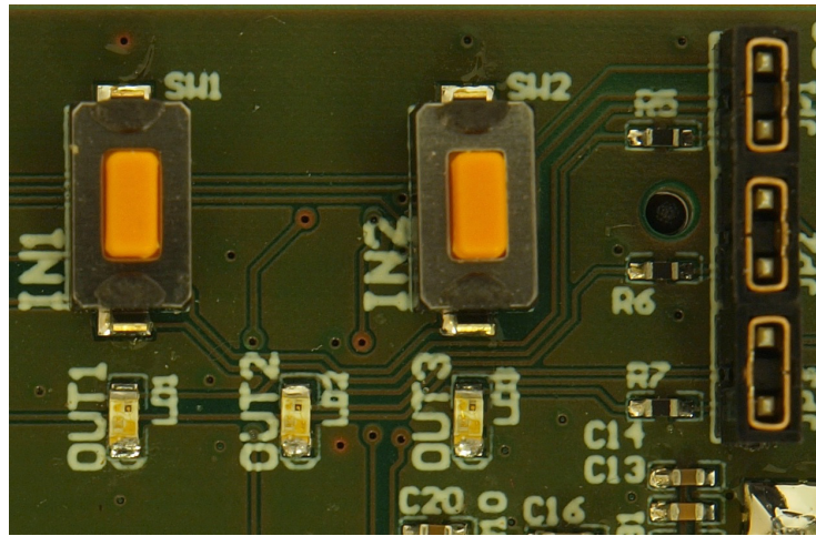
Figure 4. LEDs and buttons
