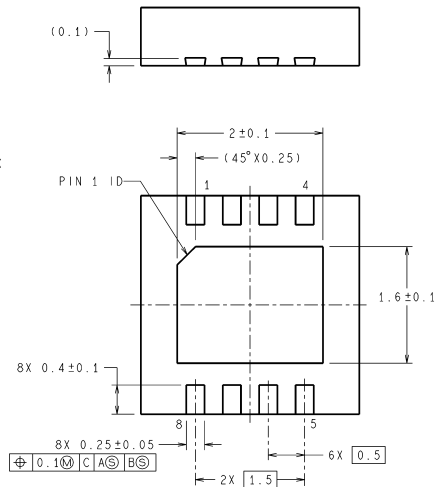
8-Lead Thin Leadless Leadframe Package NS Package Number SDA08A
