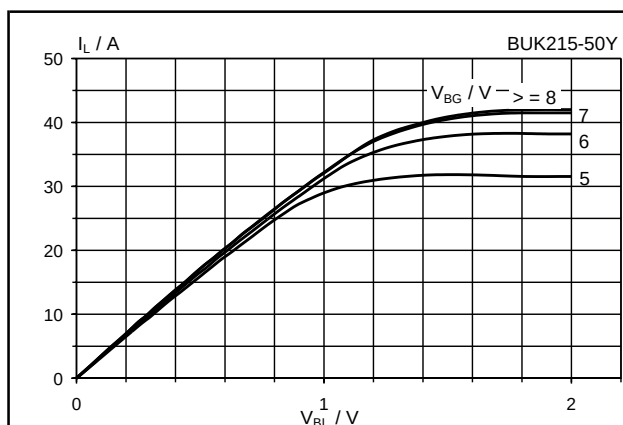
Fig.6. Typical on-state characteristics, T_j = 25 ^\circ C . I_L = f(T_j) ; parameter V_{BG} ; t_p = 250 \mu s
