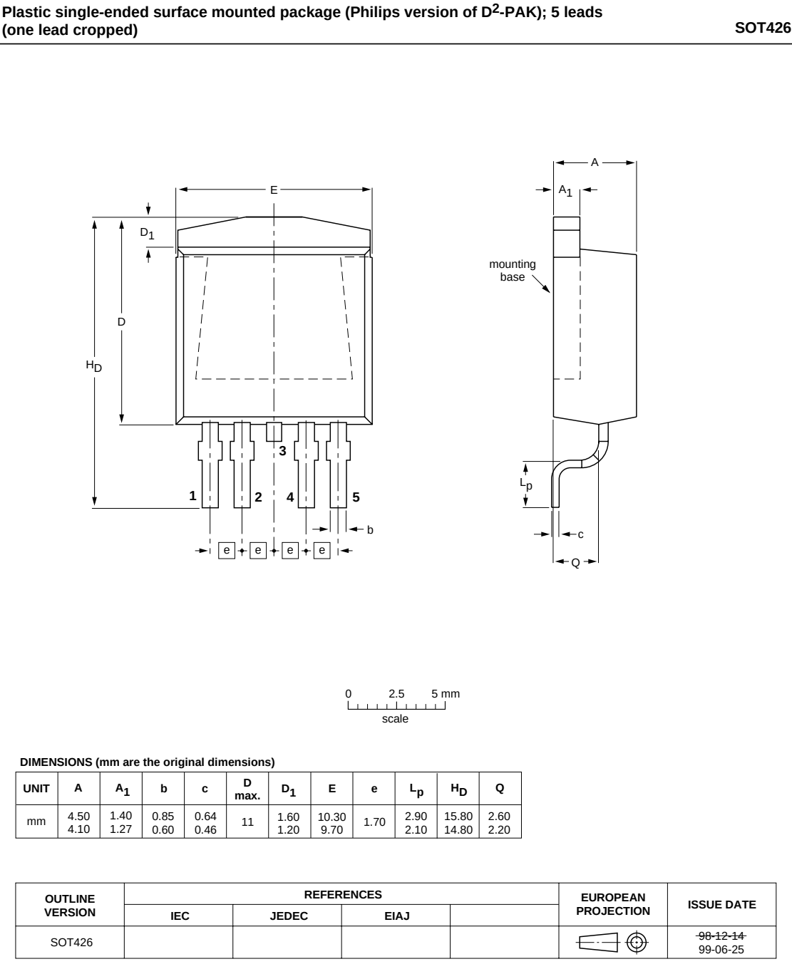
Fig.34. SOT426 surface mounting package 1 , centre pin connected to mounting base.
