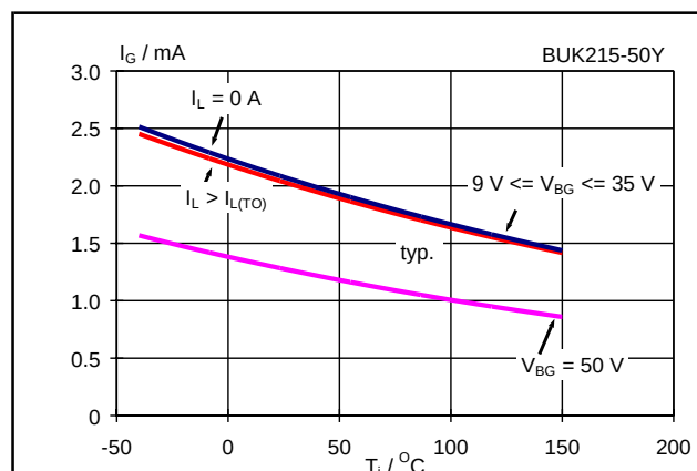
Fig.9. Typical operating supply current. I_G = f(T_j) ; parameters I_L , V_{BG} ; condition V_{IG} = 5 V
