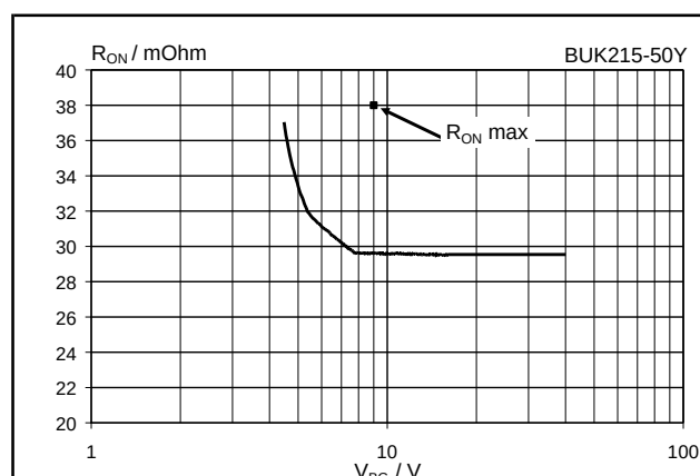
Fig.8. Typical on-state resistance, T_j = 25 ^\circ C . R_{ON} = f(V_{BG}) ; condition I_L = 10 A ; t_p = 300 \mu s
