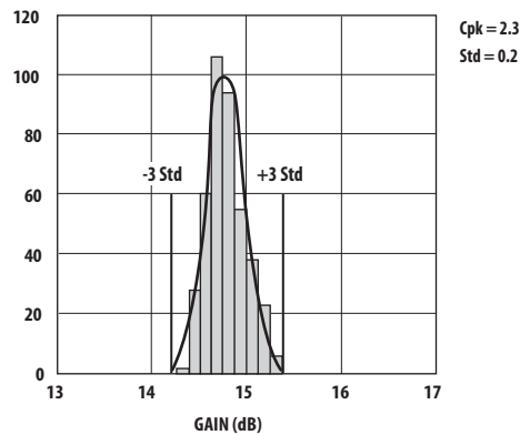
Figure 4. Gain @ 2 GHz, 4 V, 80 mA. LSL=13.5, Nominal=14.8, USL=16.5
