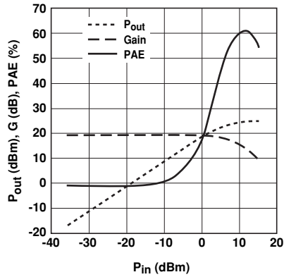
Figure 20. Swept Power Tuned for Max P_{1dB} V_{DS} = 4\text{ V} , I_{DSQ} = 80\text{ mA} , 2 GHz.
