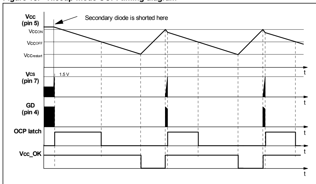
Figure 18. Hiccup-mode OCP: timing diagram
