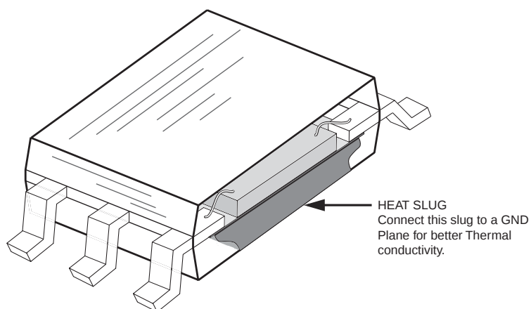
Figure 1. Cutaway view of PSOP Package
