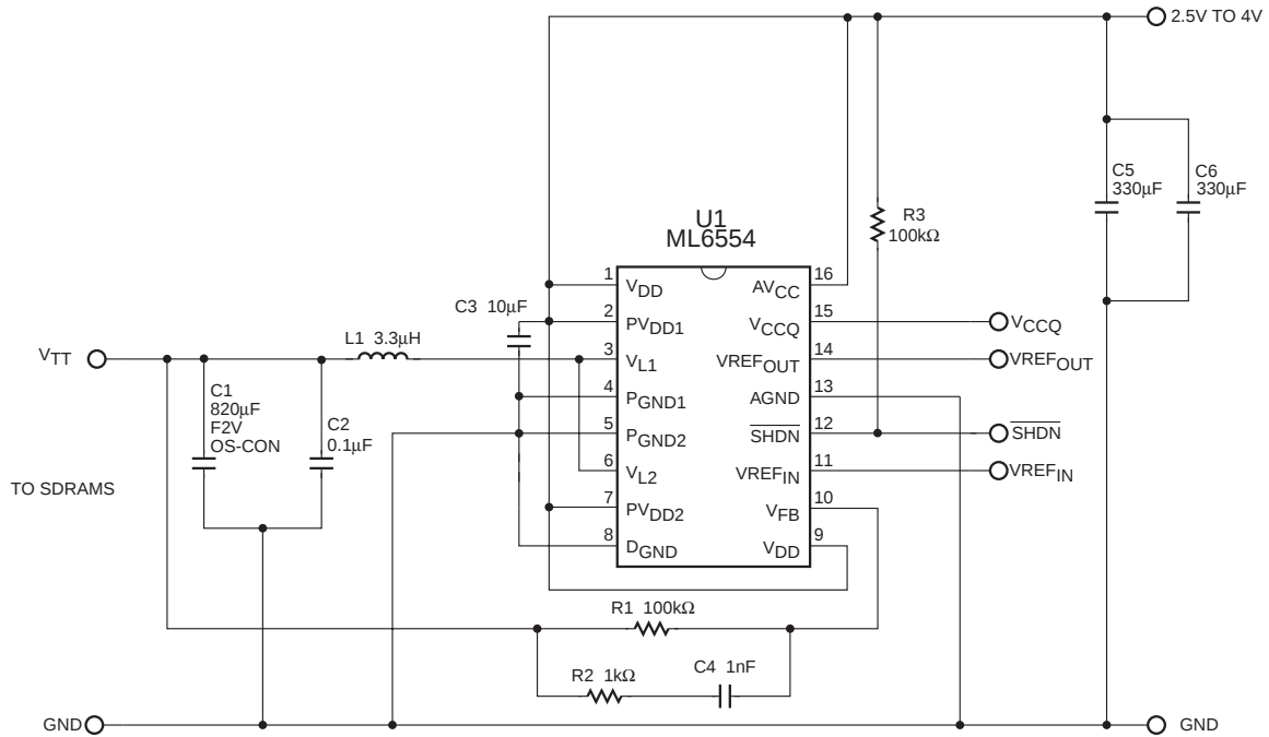
Figure 3. Alternate Application Circuit
