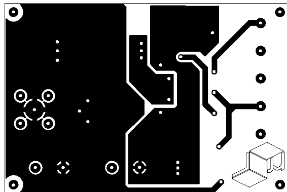
Figure 8. Bottom Layer
