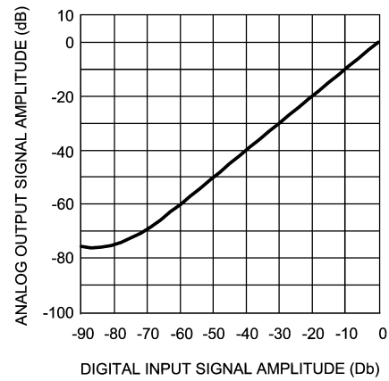
Linearity
