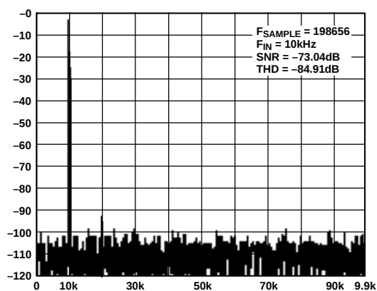
Figure 11. AD7896 FFT Plot Effective Number of Bits
