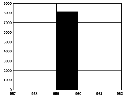
Figure 10. Histogram of 8192 Conversions of a DC Input
