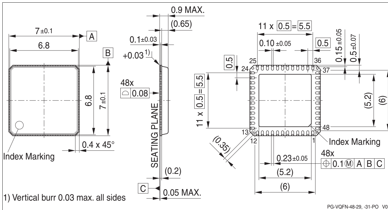
Figure 34 Package outline TLE9832QX, VQFN-48-29
