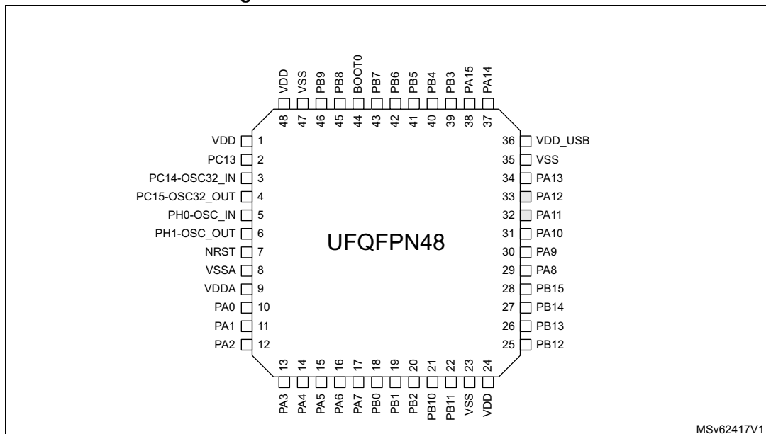
Figure 6. STM32L052x6/8 UFQFPN48
