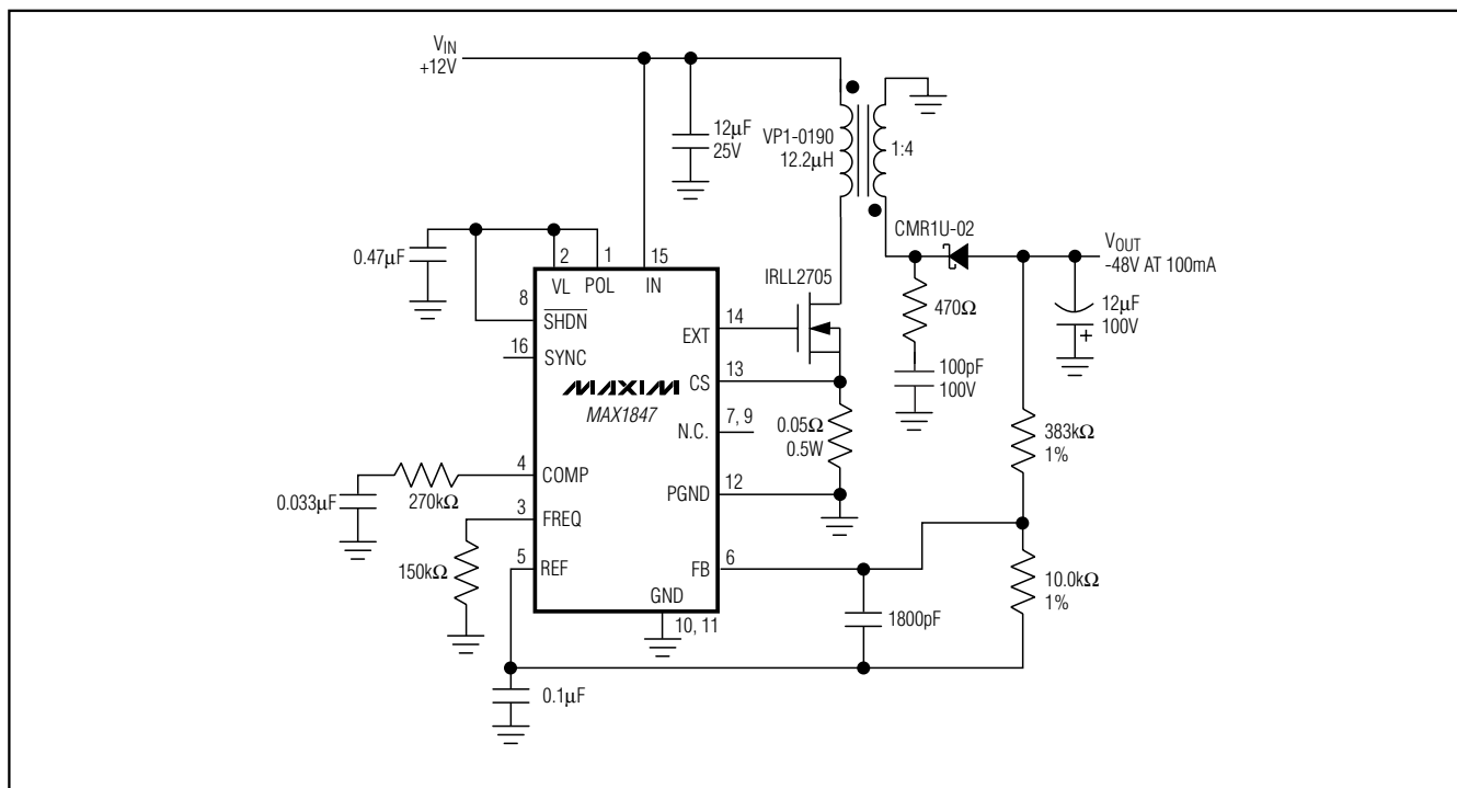
Figure 1. Using an N-Channel MOSFET (MAX1847 only)
