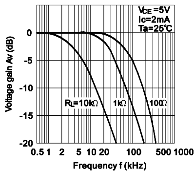
Fig.11 Frequency Response
