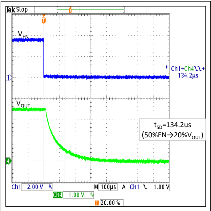
Figure 38. Shutdown ( V_{IN}=3.6V , V_{OUT}=2.5V , I_{OUT}=500mA , EN=V_{IN} \rightarrow 0 )
