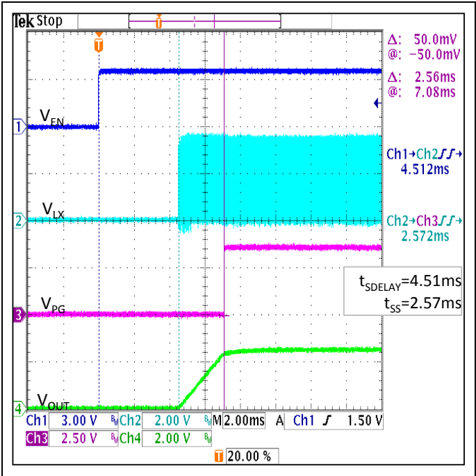
Figure 36. Startup ( V_{IN}=3.6V , V_{OUT}=2.5V , I_{OUT}=500mA , EN=0 \rightarrow V_{IN} )
