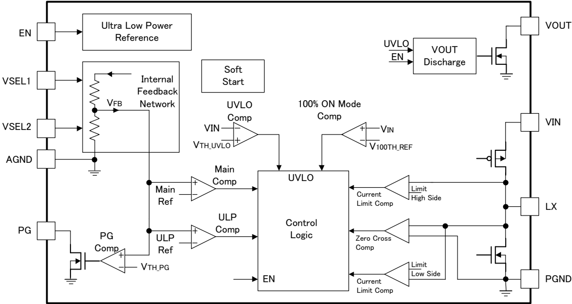
Figure 3. Block Diagram
