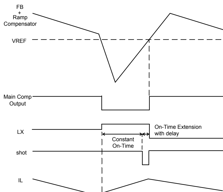
Figure 6. On-Time Extension
